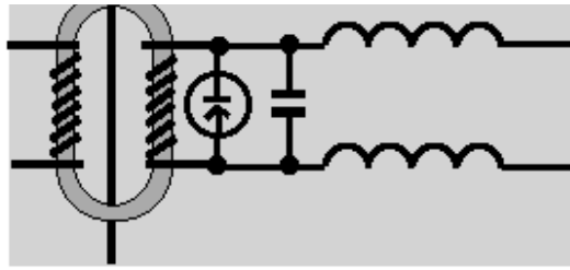
FIG.11 COMPUTER ROOM HARDENED AGAINST EM ATTACK
