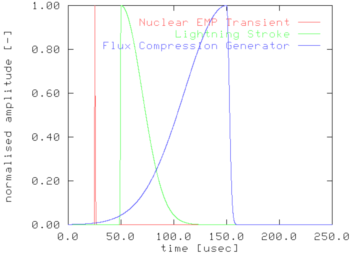
Fig.1 Typical Electromagnetic Pulse Shapes
