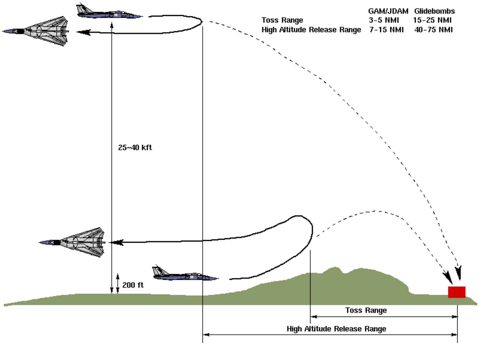
FIG.10 DELIVERY PROFILES FOR GPS/INERTIAL GUIDED WEAPONS
